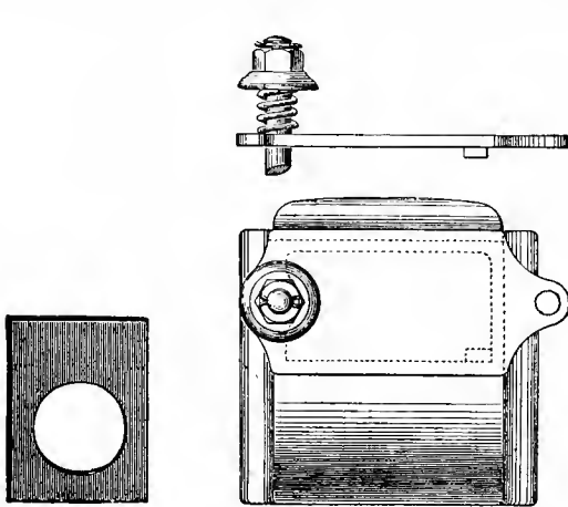
Fig 5154 DUST-GUARD.
